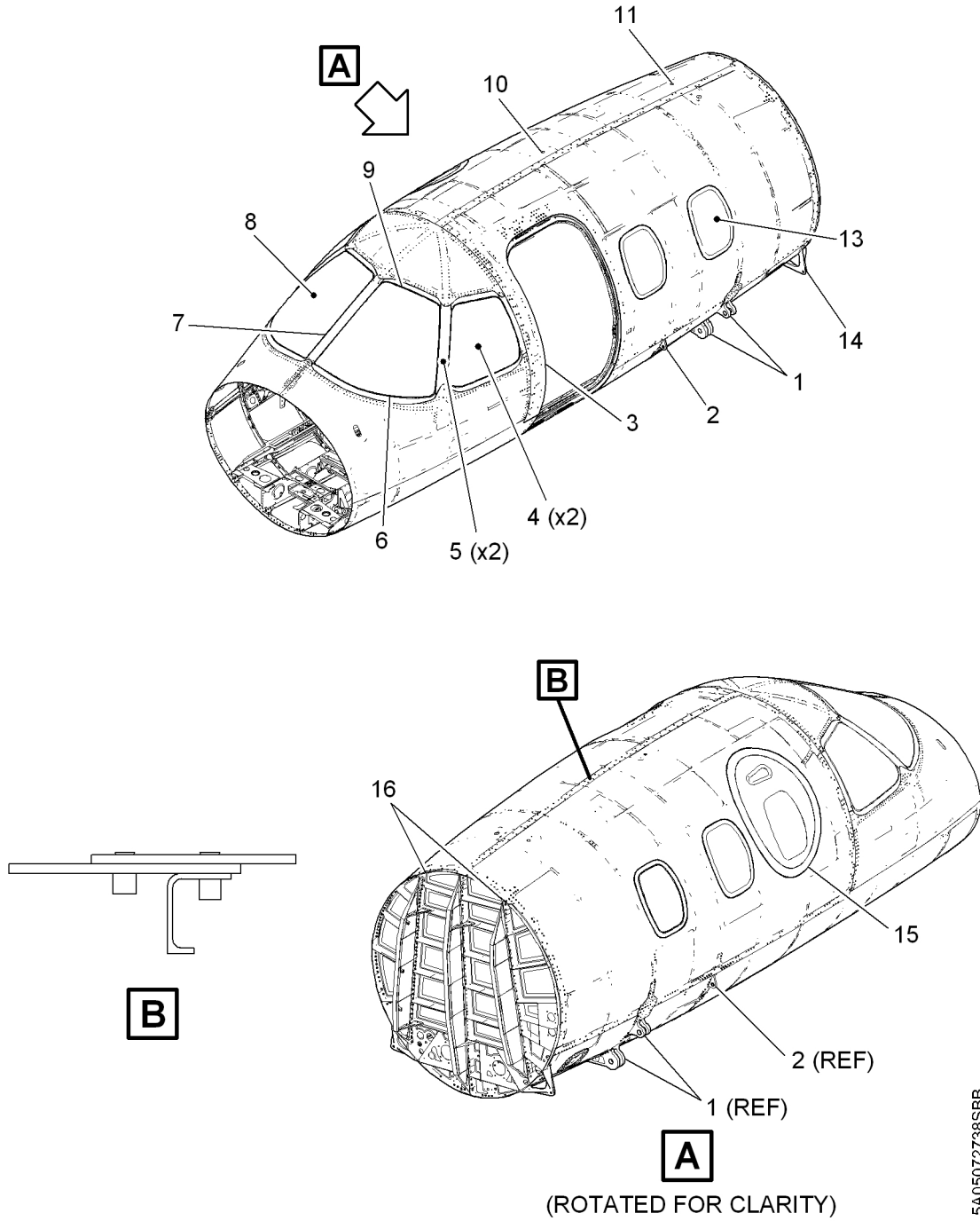
Fuselage Structural Inspection Figure 1 (Sheet 1 of 2)
