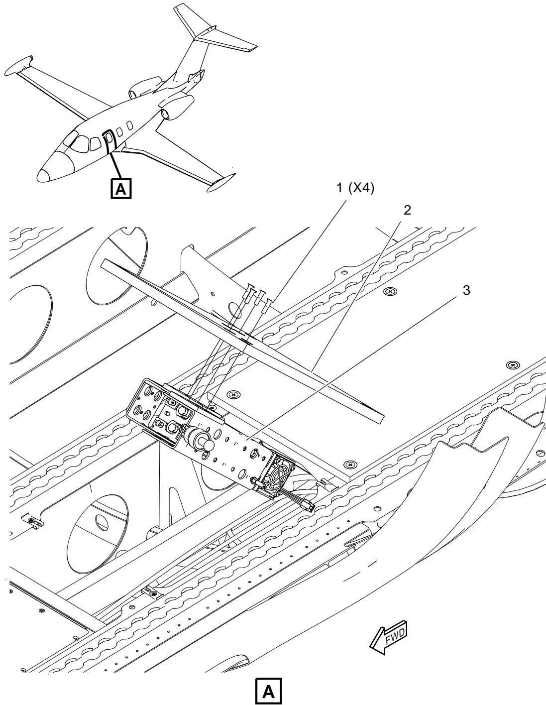
GPS 3 Mount - Removal/Installation Figure 401 (Sheet 1 of 2)
