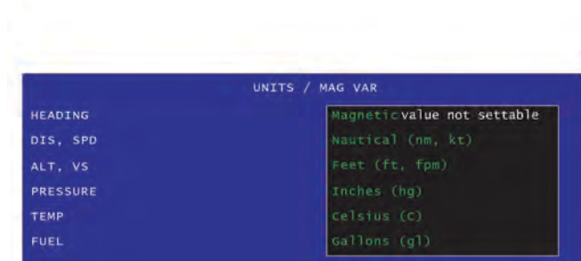
GPS 400W Panel – UNITS / MAG VAR Settings Figure 214 (Sheet 1 of 1)
