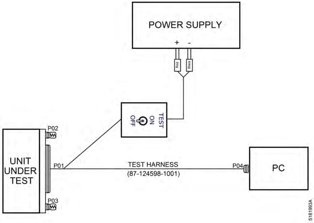
Test Setup Figure 201 (Sheet 1 of 1)
