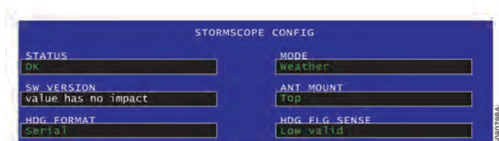
GPS 400W Panel – STORMSCOPE CONFIG Settings Figure 210 (Sheet 1 of 1)
