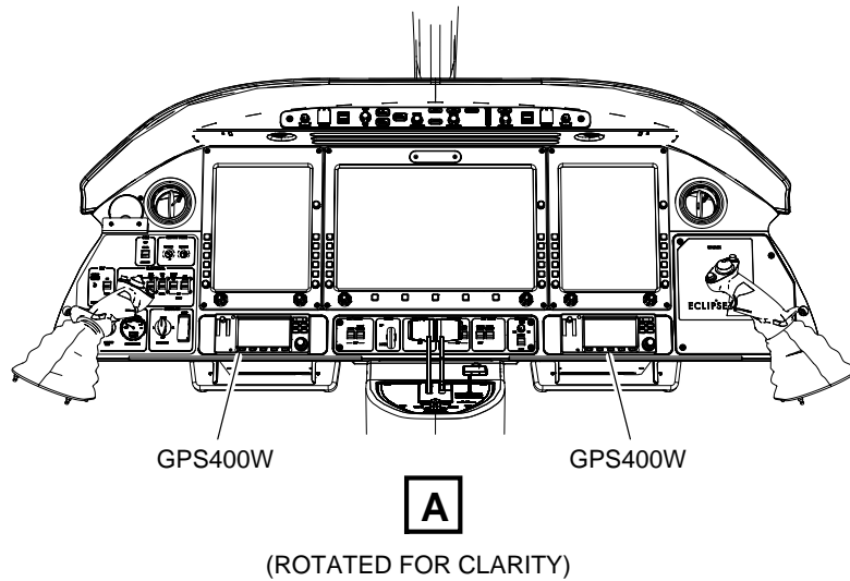
GPS — Combination Antenna Location Figure 1 (Sheet 1 of 1)
