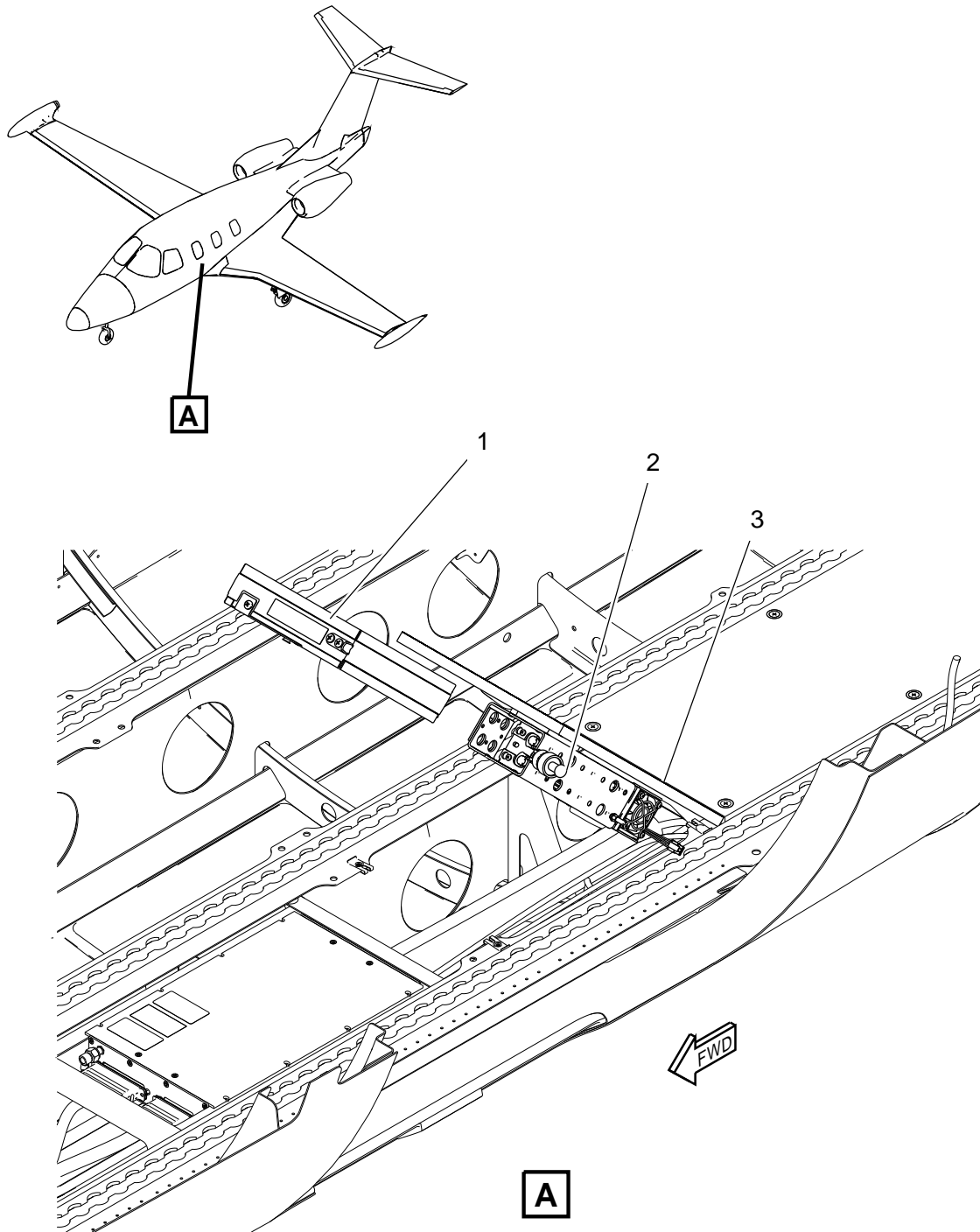
GPS 3- Removal/Installation Figure 401 (Sheet 1 of 1)
