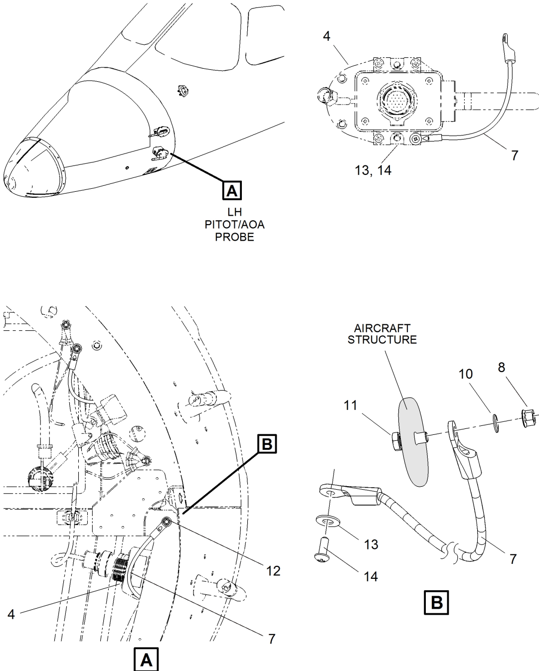
Pitot/AOA Probes - Removal/Installation Figure 401 (Sheet 2 of 4)
